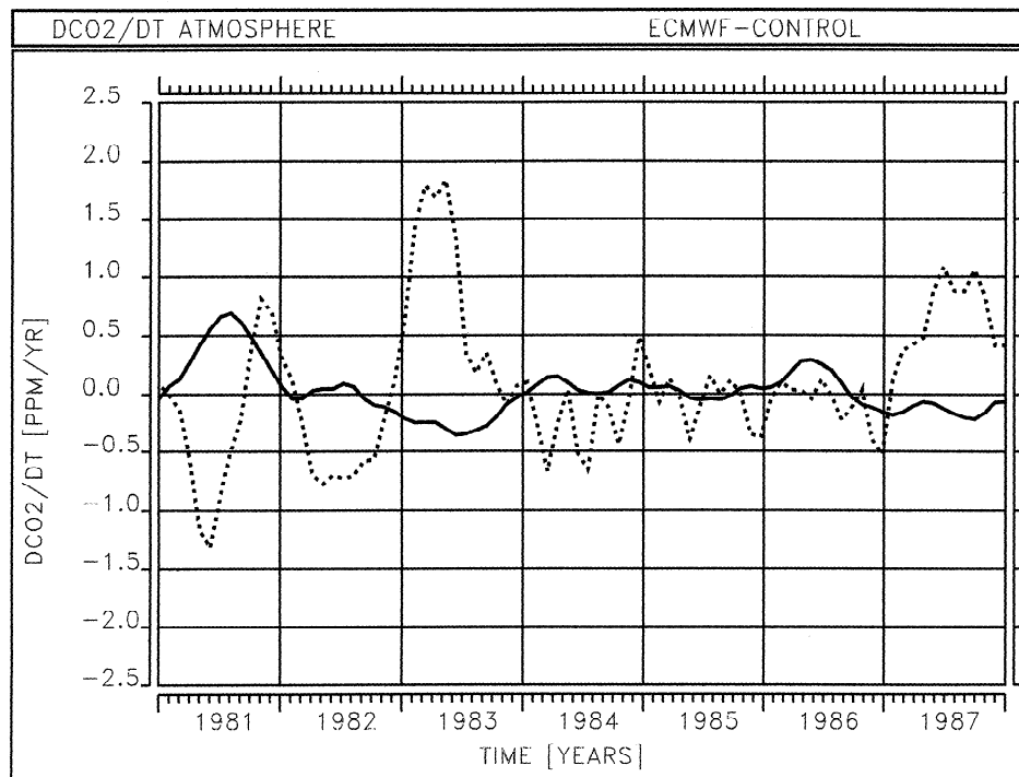
Figure 11. Time series of the 5-month running mean of the difference from the atmospheric \text{CO}_2 growth rate between experiment and control run (solid) compared with the anomaly of the atmospheric \text{CO}_2 growth rate after Keeling et al. [1989] (dashed) in Figure 1.
