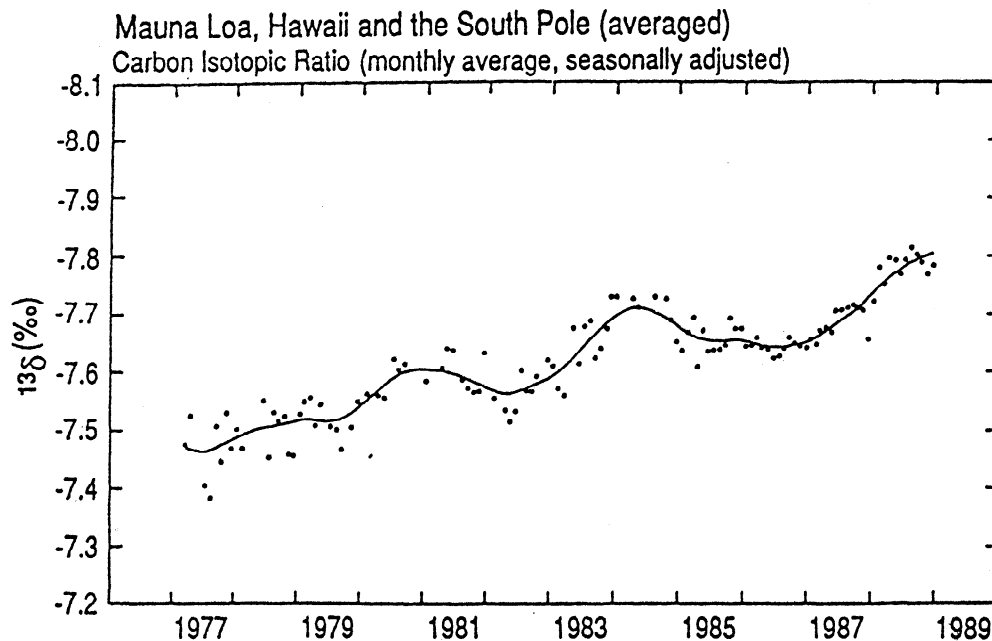
Figure 2. Seasonally adjusted record of \delta^{13}\text{C} of atmospheric CO 2 in ‰: observations from Mauna Loa Observatory, Hawaii, and the South Pole combined by averaging [ Keeling et al., 1989, Figure 25, p. 182 ].
