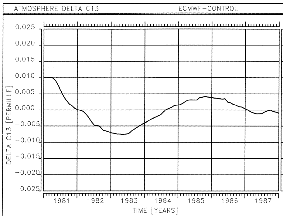
Figure 12. Time series of interannual fluctuations of the global atmospheric \delta^{13}\text{C} in ‰: model results from experiment minus control run.
