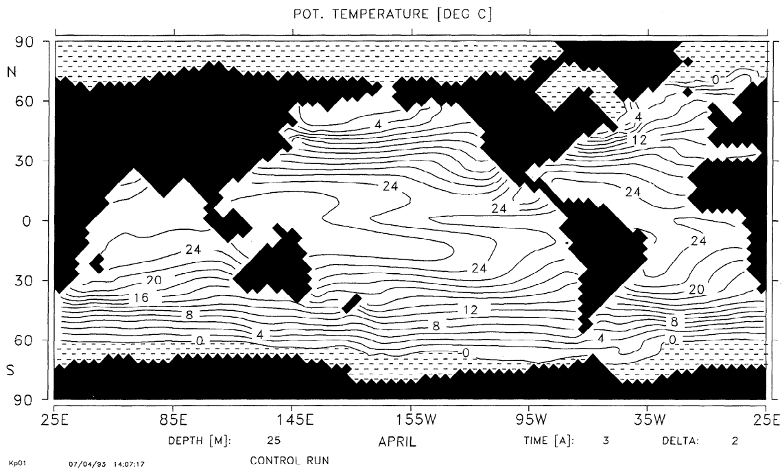
Figure 4. Control run, April: sea surface temperature (SST) (contour interval 2^{\circ}\text{C} ).
